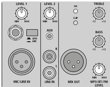
② PAK-8DMP/-10DMP Connections, controls
